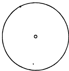
EARTH, AND MOON'S ORBIT.
